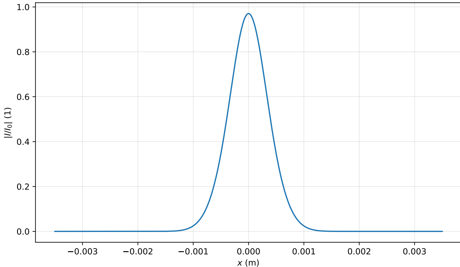
Intensity profile I(x, y = 0, z = 0.796m)/I_0 , P_{in}=0.3P_{cr} , artificial time
